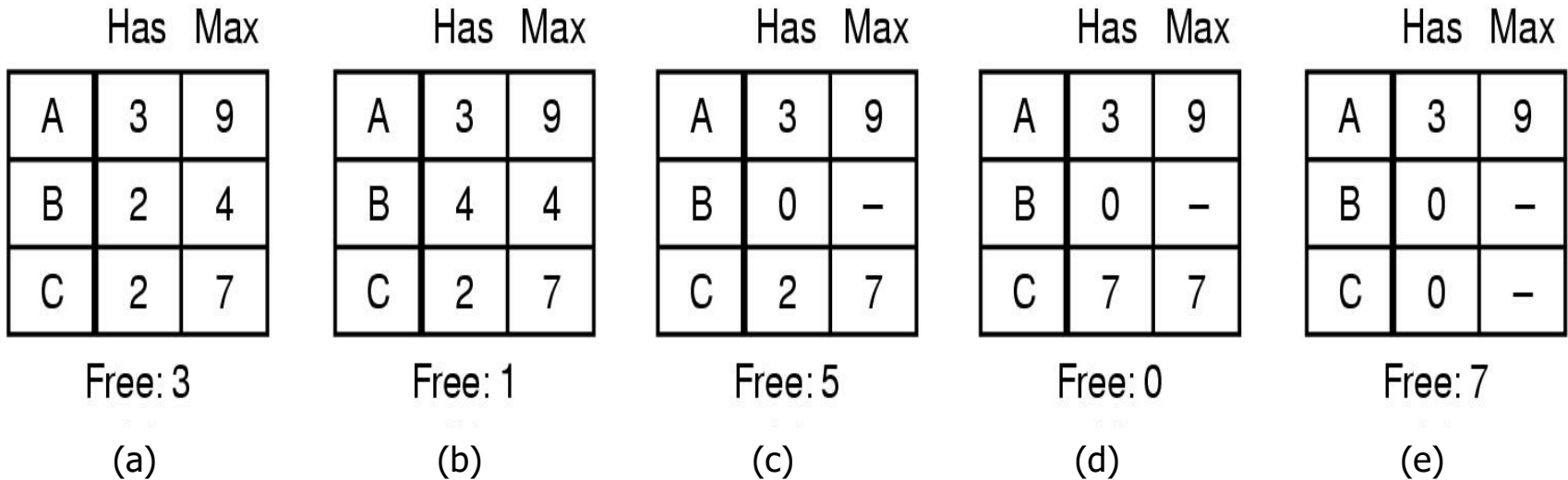
Figure: Demonstration that the state in (a) is safe
