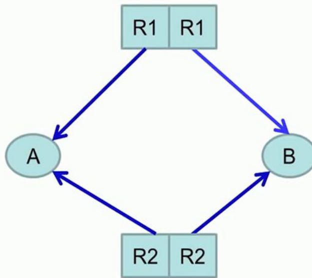
No Deadlocks
