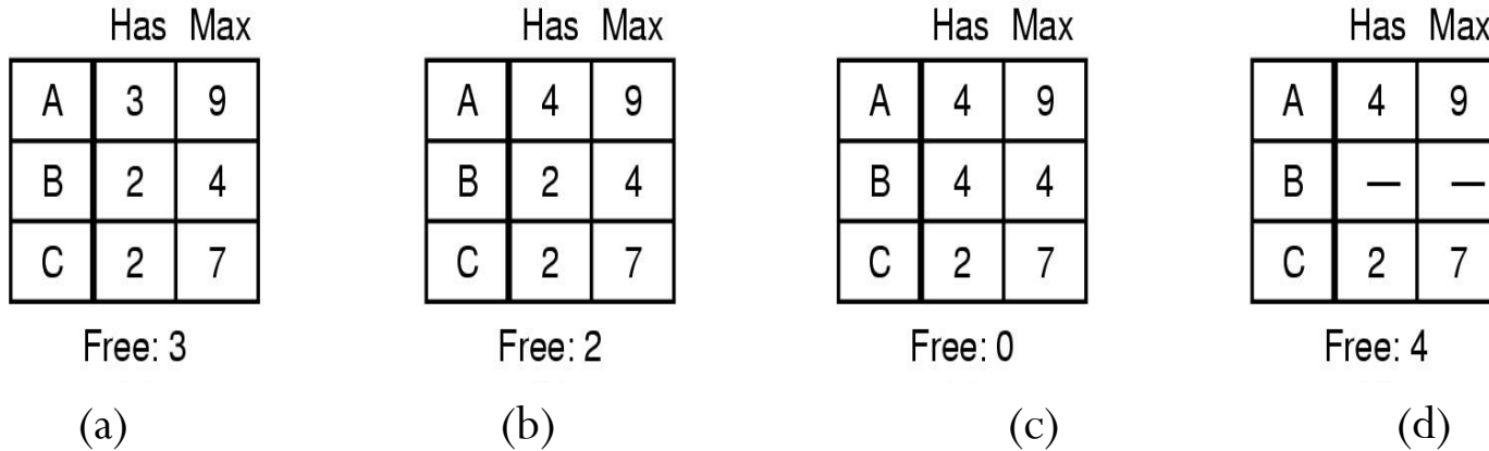
Figure: Demonstration that the state in (b) is not safe
