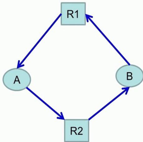
A deadlocked state
